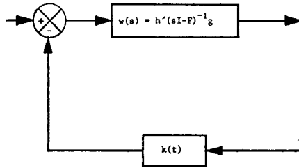
Fig. 1. Closed-loop system.
